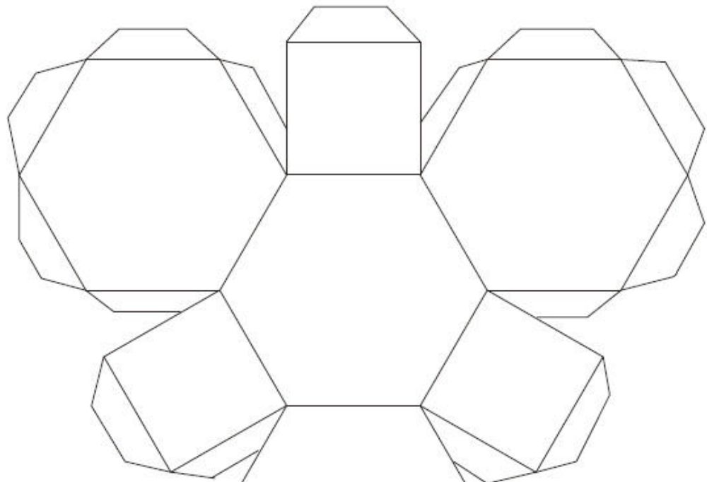
Truncated Octahedron
